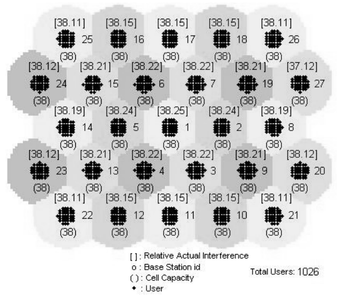
Fig. 11. Maximum network capacity of 1026 using actual interference with best case non-uniform user distribution.
