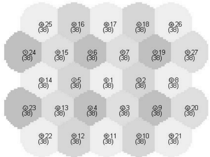
Fig. 12. 2-D Gaussian approximation of users densely clustered around the BSs. \sigma_1=\sigma_2=100 , \mu_1=\mu_2=0 . The maximum number of users is 1026.
